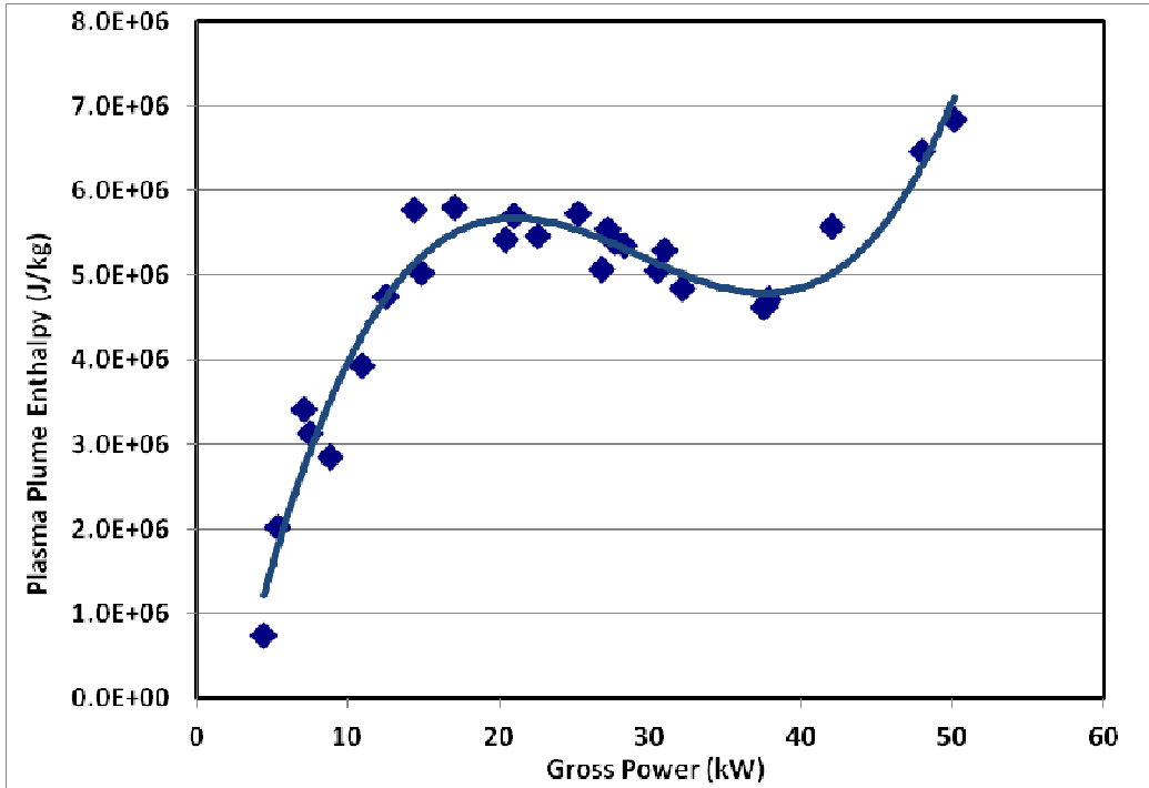
Figure 2 – Gross Power vs. Plasma Plume Enthalpy for compact coaxial plasma torch (Minigun) with pure argon as the plasma forming gas.
