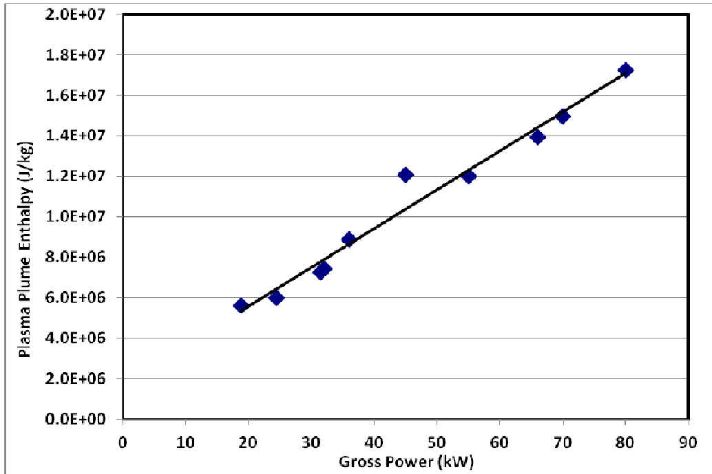
Figure 5 – Gross Power vs. Plasma Plume Enthalpy for reverse polarity high polarity plasma torch with pure argon as the plasma forming gas.
