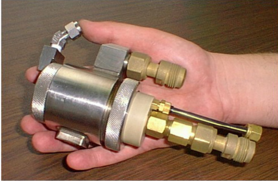
Figure 1 – A picture of the assembled compact coaxial plasma torch (Minigun)
