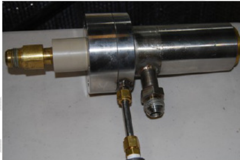
Figure 4 – A picture of the assembled reverse polarity high enthalpy plasma torch
