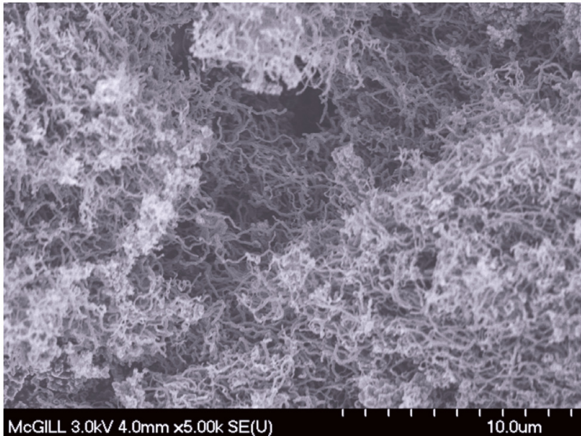
Figure 7 – Carbon nanotubes produced with an RPT torch (Photo courtesy of McGill University)
