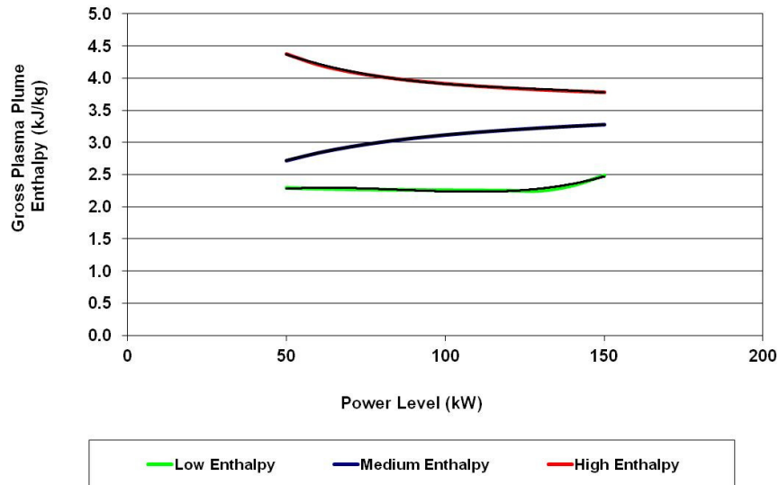
Figure 8 – Gross Power vs. Plasma Plume Enthalpy for air plasma torch.
