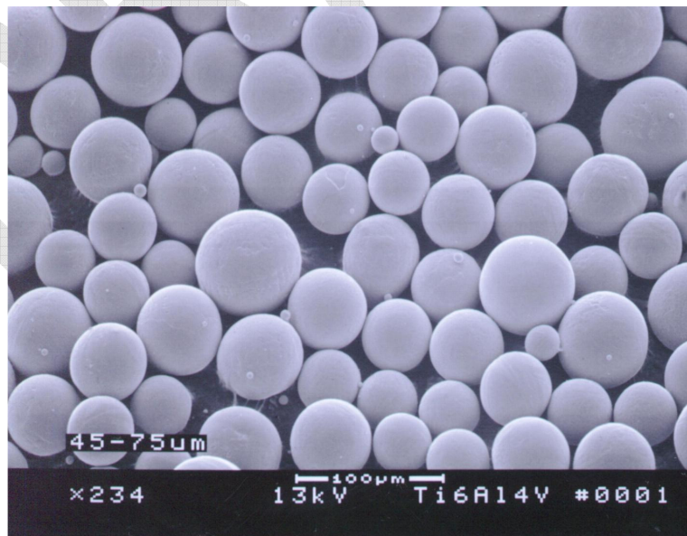
Figure 6 – Spherical metallic powders produced using RPT™ plasma torch.
