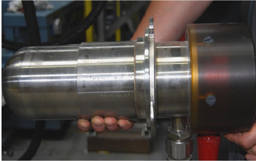
Figure 7 – A picture of the assembled air plasma torch
